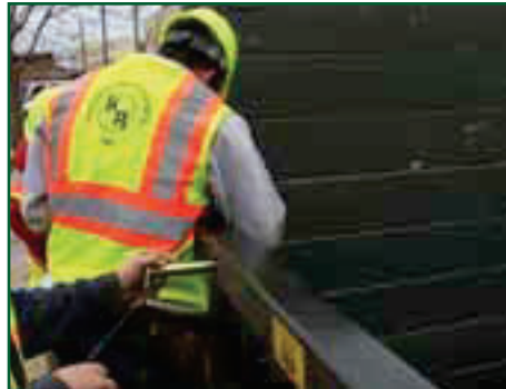
4. Spreaders are pinned in place
